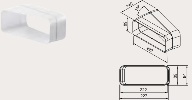
Tubo curvo horizontal 15
